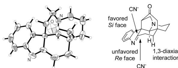
Figure 3. Stereochemical course in addition of hydrogen cyanide to the imine (±)- 2 .
