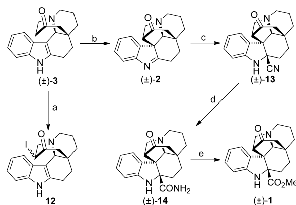
Scheme 2. Reagents and conditions: a) LiHMDS, THF, −78 °C, 30 min, then I 2 , −78 °C to RT, 35–78% yields; b) LiHMDS, THF, −78 to −40 °C, 30 min, then I 2 , −40 °C to RT, 77%; c) TMSCN, MeOH, THF, 50 °C, 96%; d) K 2 CO 3 , H 2 O 2 , MeOH; e) HCl, MeOH, 45% yield for 2 steps. HMDS = hexamethyldisilazide, TMS = trimethylsilyl.
