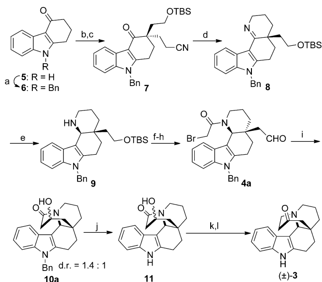
Scheme 1. Reagents and conditions: a) BnBr, NaH, DMF, 83%; b) LDA, ICH 2 CH 2 OTBS, THF, 65%; c) t BuOK, acrylonitrile, t BuOH, THF, 70%; d) NiCl 2 ·6H 2 O, NaBH 4 , NH 2 NH 2 ·H 2 O, NaOH, EtOH; e) Pd/C, H 2 , EtOH, 90% yield for 2 steps; f) 2-bromoacetyl chloride, CH 2 Cl 2 , NaOH; g) HBr, THF; h) 0.05 mol% TPAP, NMO, CH 2 Cl 2 , 69% yield for 3 steps; i) SmI 2 , THF, 78%; j) Na, liquid ammonia, THF, t BuOH; k) BH 3 ·THF; l) Py·SO 3 , DMSO, Et 3 N, CH 2 Cl 2 , 52% yield from 10a . DMSO = dimethylsulfoxide, DMF = N,N -dimethylformamide, LDA = lithium diisopropylamide, NMO = N -methylmorpholine- N -oxide, TBS = tert -butyldimethylsilyl, THF = tetrahydrofuran, TPAP = tetrapropylammonium perruthenate.
